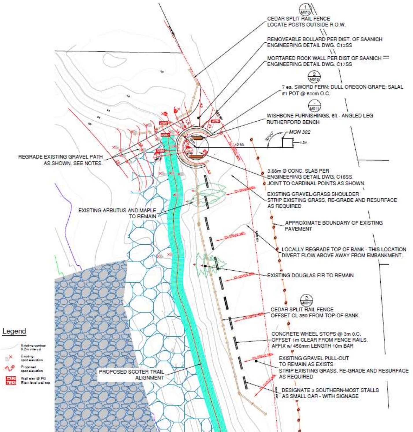
TRAILHEAD - PLAN VIEW SCALE 1:150
